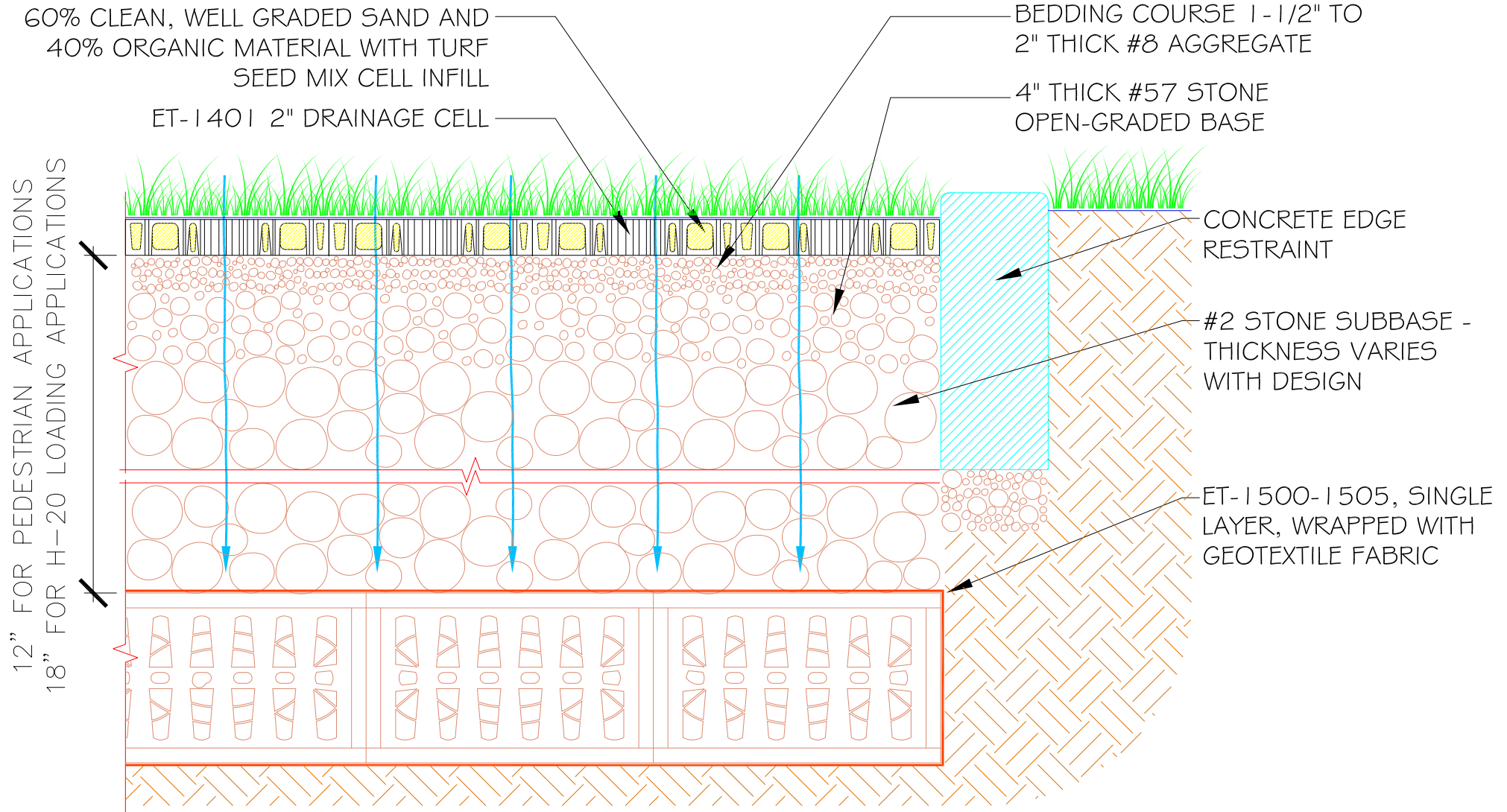
CONCEPT DRAINAGE CELL TURF PAVER WITH TANKS INSTALLATION SECTION
